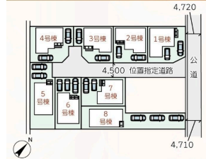
Block Plan
